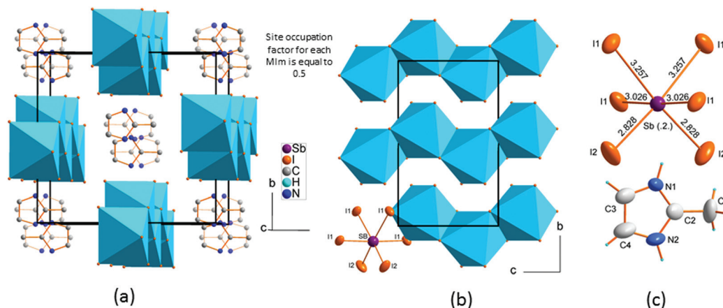
Fig. 3 Crystal structure of (2-MIm)SbI 4 in phase I, T = 330 K. (a) The crystal packing with disordered 2-MIm + counter-cations, (b) zig-zag chains expand along the c -direction, (c) the basic units in ellipsoid representation.
