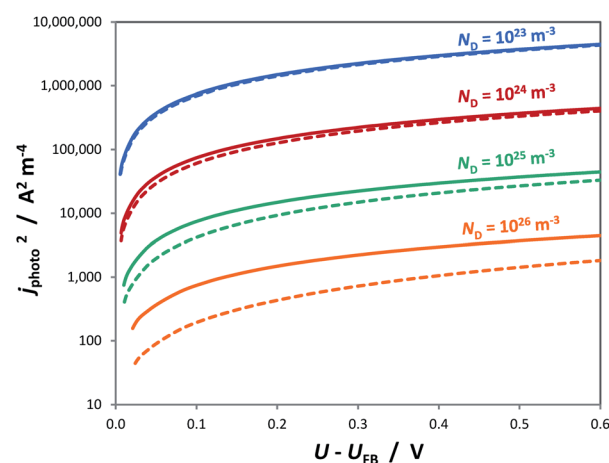
Fig. 7 Square of the photocurrent predicted by the Gärtner-Butler equation using \alpha_{\lambda} = 1.6 \times 10^7 \text{ m}^{-1} , I_{0,\lambda} = 3.6 \times 10^{21} \text{ m}^{-2} \text{ s}^{-1} , \epsilon_r = 80 , n_0 \approx N_D (for various doping levels), p_0 \approx 0 , C_H = 0.2 \text{ F m}^{-2} and U_{\text{FB}} = 0 for the cases of U - U_{\text{FB}} = \Delta\phi_{\text{SC}} + \Delta\phi_{\text{H}} (---) and U - U_{\text{FB}} \approx \Delta\phi_{\text{SC}} (—).
