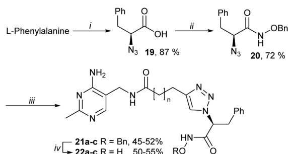
Scheme 3 Synthesis of hydroxamates 22a–c . Reagents and conditions: (i) triflyl azide, CuSO 4 ·5H 2 O, K 2 CO 3 , MeOH, H 2 O, RT; (ii) CDI, NH 2 OBn·HCl, THF, DMF, RT; (iii) 11a–c , CuSO 4 ·5H 2 O, sodium ascorbate, t -BuOH, H 2 O, 40 °C; (iv) BCl 3 , DCM, RT. For all compounds: a n = 1, b n = 2, c n = 3.
