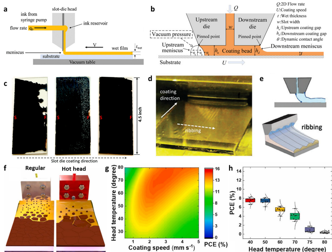
Fig. 8 (a) Schematic diagram of the slot-die coating equipment. 99 Copyright 2024, Wiley-VCH GmbH. (b) Schematic diagram fluid mechanics models and core parameters in slot-die coating. 103 Copyright 2016, American Institute of Chemical Engineers. (c) Images of slot-die coated perovskite thin films under different combination of ink supply rate and coating speed. From left to right: too fast, too slow and balanced supply. 104 (d) The image and (e) schematic illustrations of ribbing defects during slot-die coating. 99 Copyright 2024, Wiley-VCH GmbH. (f) Schematic diagram of slot die coating of perovskite films using 150 °C substrate-heating (left) and 150 °C substrate-heating/75 °C substrate-heating (right). (g) Color map of PCEs at the different head temperatures versus slot-die coating speeds. (h) Only-head heating with various temperatures. 105 Copyright 2022, Elsevier B.V.
