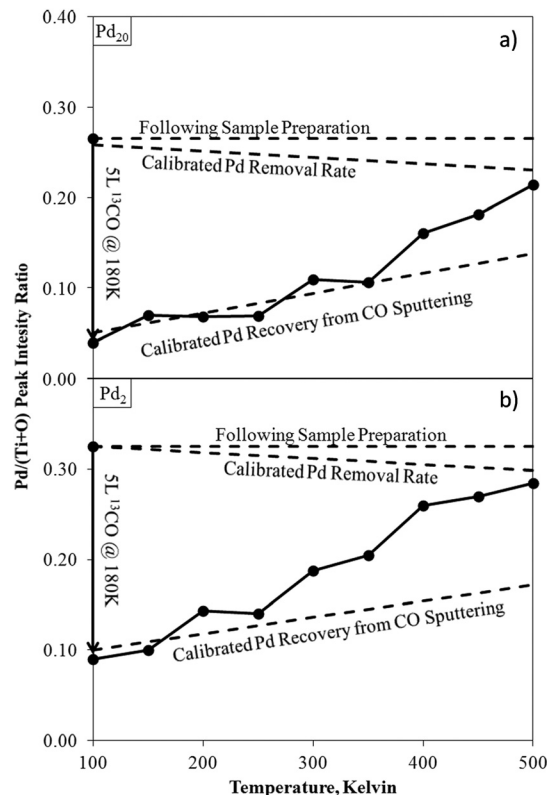
Fig. 12 Pd/(Ti + O) ISS intensity ratios for Pd 20 /TiO 2 (a) and Pd 2 /TiO 2 (b) as-deposited, after exposure to CO at 180 K, and during temperature ramping. Calibrated rates for recovery of Pd from ISS sputtering. 171 Calibration lines account for unintended sputtering effects from the ISS experimental conditions selected for this analysis. Deviations from this calibration indicate a changing surface structure (desorption of CO).
