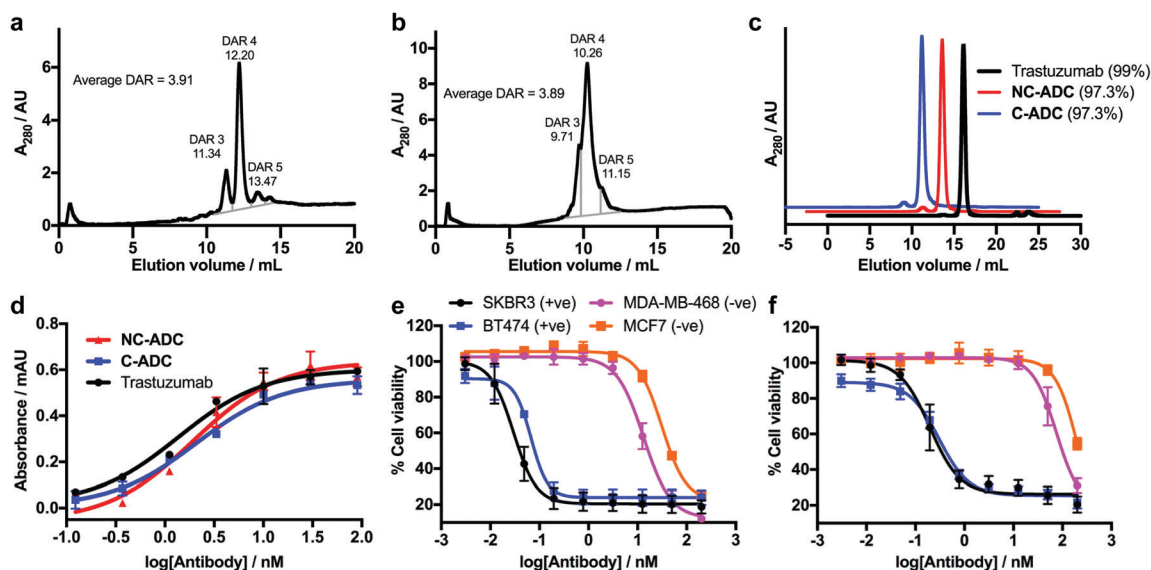
Fig. 2 In vitro characterisation of DVP ADCs. (a) HIC trace of C-ADC , (b) HIC trace of NC-ADC , (c) SEC traces of trastuzumab, NC-ADC and C-ADC , (d) HER2 ELISA of trastuzumab, NC-ADC and C-ADC . Error bars represent the standard deviation of biological quadruplicates, (e) cell viability of C-ADC against HER2-positive (+ve) and HER2-negative (–ve) cell lines, and (f) cell viability of NC-ADC against the same cell lines. Viability data shows the mean of three independent replicates and error bars represent S.E.M.
