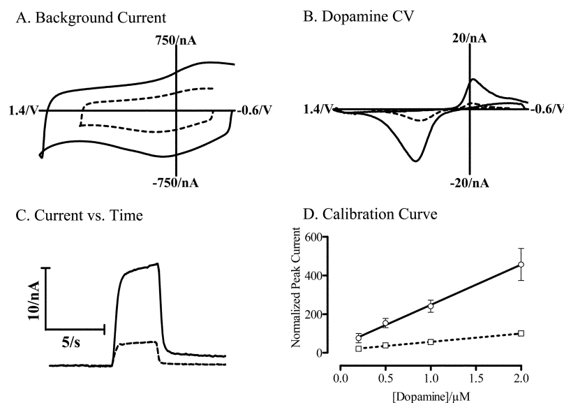
Fig. 1 In vitro characterization of waveforms. The traditional waveform ( -0.4 V to 1.0 V, 300 V s^{-1} ) is shown in dashed lines, while the extended waveform ( -0.6 V to 1.4 V, 400 V s^{-1} ) is shown in solid lines. A: Background cyclic voltammograms for the two potential limits at the same electrode recorded in TRIS buffer solution, pH 7.4. B: Background-subtracted cyclic voltammograms for 1 \mu\text{M} dopamine. C: Response to a bolus dopamine injection, in which the peak oxidation current of each cyclic voltammogram is plotted vs. time. D: Calibration curve for dopamine ( n = 6 ). Due to variations between electrodes, each electrode response was normalized to the response for 2 \mu\text{M} dopamine with the traditional waveform. The error bars represent the standard deviation.
