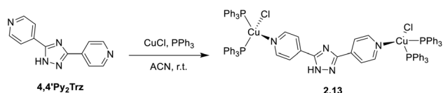
Scheme 17 Synthesis of 2.13.
