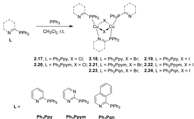
Scheme 20 Synthesis of 2.17–24 .
