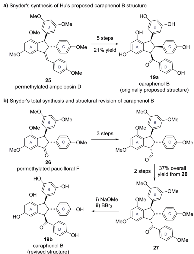
Scheme 3 (a) Snyder's synthesis of Hu's proposed caraphenol B structure. (b) Snyder's total synthesis and structural revision of caraphenol B.
