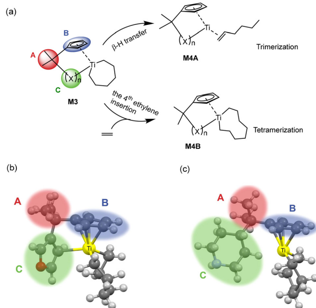
Fig. 1 A schematic diagram of ethylene oligomerization starting from the metallacycle intermediate: (a) the chain termination resulting in the trimerization product and chain propagation for further oligomerization or even polymerization based on the metallacycle intermediate structure, and the three-dimensional schematic diagrams of two types of specific active species M3 shown in (b) and (c), respectively.
