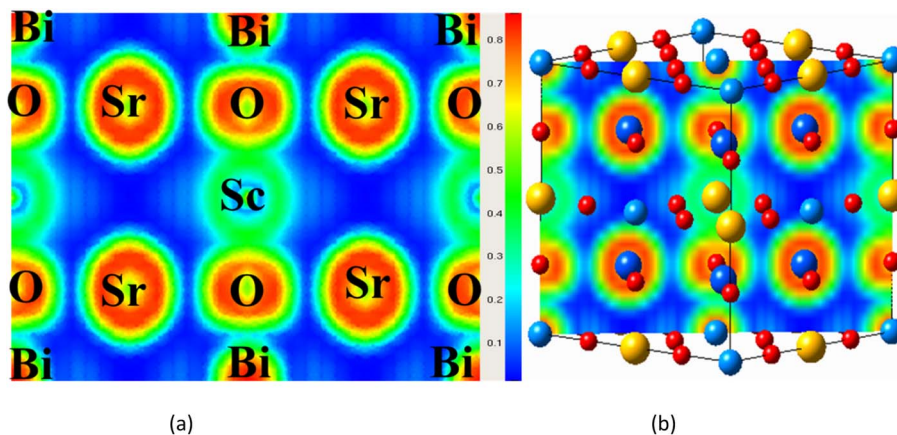
Fig. 6 (a and b) Electron localization function profile of \text{Sr}_2\text{ScBiO}_6 along 110 plane.
