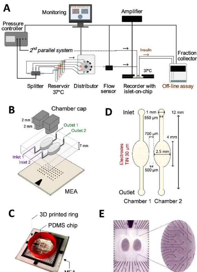
Fig. 1 Overview of the microfluidic system and of the design of the islets-on-chip. (A) Front view of the automated microfluidic MEA system and fraction collector. (B) Exploded view of the microfluidic chip. PDMS chambers are bonded to the MEA by O_2 plasma and closed with 3D-printed caps. The reference electrode is given in black. (C) Image of the assembled microfluidic chip with 3D-printed media containment ring. (D) Drawing of the channels and chambers on the electrodes and corresponding dimensions. The TiN electrodes ( \varnothing 30 \mu m) were spaced 500 \mu m apart. (E) Image of the chambers with the electrodes in titanium nitride (TiN).
