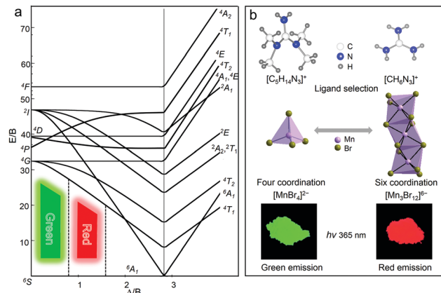
Fig. 4 (a) Tanabe–Sugano (TS) energy diagram of 3d^5 electron orbital of Mn^{2+} . (b) Modifying the coordination units of Mn^{2+} by selecting different organic ligands to modulate the photoluminescence properties.
