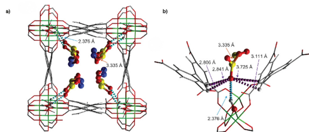
Fig. 3 (a) View of the crystal structure of NOTT-300.4.0- \text{SO}_2 obtained from Rietveld refinement of data on \text{SO}_2 -loaded material at 1.0 bar. The adsorbed \text{SO}_2 molecules in the void are highlighted using a ball-and-stick representation. The sulfur atom of the second site of \text{SO}_2 is highlighted in blue. (b) Detailed view of the OH and CH contact with \text{SO}_2 molecules in a distorted pocket-like cavity. (Aluminum, green; carbon, grey; oxygen, red; hydrogen, white; sulfur, yellow.) (Reprinted (adapted) with permission from ref. 114 Copyright (2012) Springer Nature).
