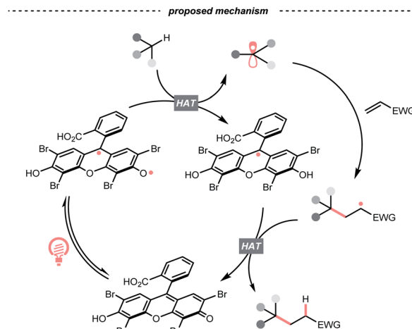
Scheme 11 Eosin Y-catalysed \text{C}(\text{sp}^3) radical generation.
