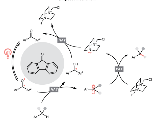
Scheme 10 Ketone-catalysed \text{C}(\text{sp}^3) -H fluorination.
