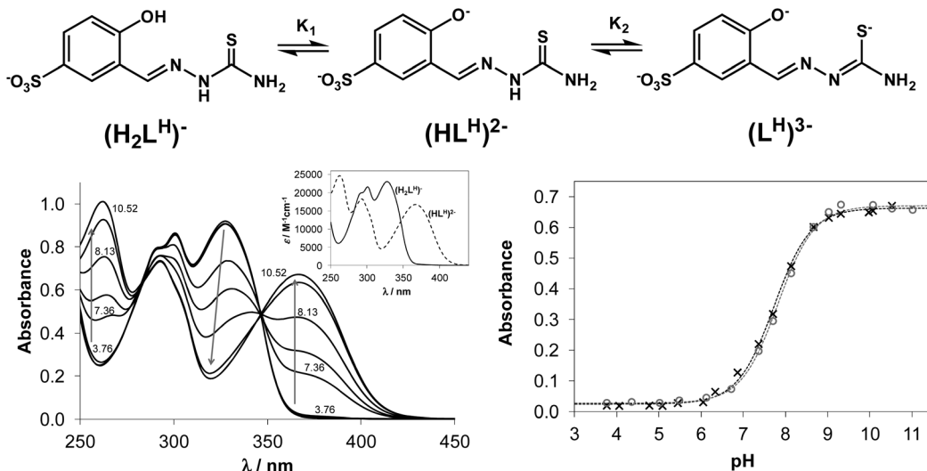
Fig. 1 (Top) Proton dissociation steps of 5-sulfonato-salicylaldehyde TSC ( \text{H}_2\text{L}^{\text{H}} ). (Bottom left) Representative UV-vis absorption spectra of \text{NaH}_2\text{L}^{\text{H}} ( C_{\text{ligand}} = 4.0 \times 10^{-5} \text{ M} ) at different pH values. Inset shows the molar absorbance spectra of the individual species ( \text{H}_2\text{L}^{\text{H}} ) and ( \text{HL}^{\text{H}} ) ^{2-} obtained by the deconvolution of the recorded spectra. (Bottom right) Dependence of the absorbance of \text{NaH}_2\text{L}^{\text{H}} (x) and \text{NaH}_2\text{L}^{\text{Me}} (o) at 363 nm from pH together with the simulated curves (dashed lines) ( C_{\text{ligand}} = 3.9 \times 10^{-5} \text{ M} ).
