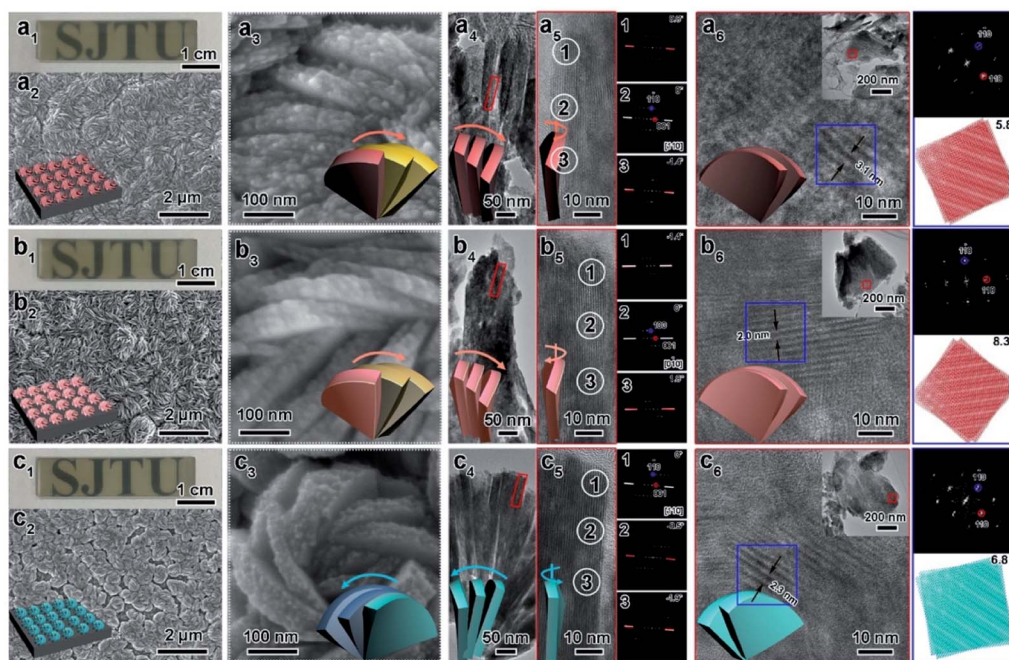
Fig. 3 Photograph, SEM images, TEM images, FDs, and corresponding models of CMBF D-Sor (a), CMBF L-Idi (b), and CMBF D-Alt (c) with different views. The synthetic molar composition was 0.5 DSA: 0.5 Bi(NO 3 ) 3 ·5H 2 O: 0.5 NaBr: 287 EG: 222 H 2 O: 7.5 × 10 −4 NaOH.
