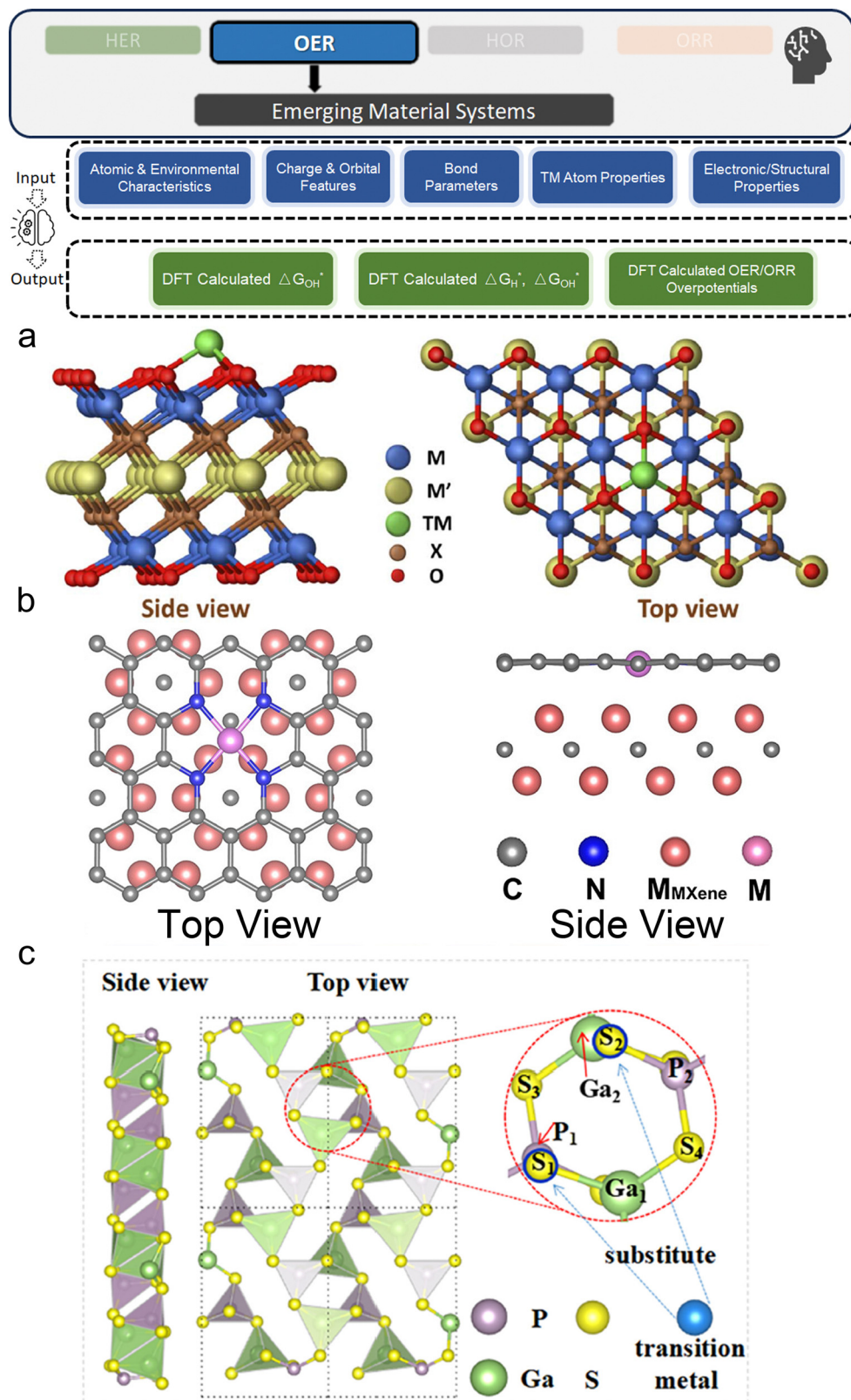
Fig. 22 (a) Schematic illustration of the side and top views of the investigated O-terminated M_2M'X_2O_2 -type doped MXenes. TM acts as the active site for the adsorption of intermediates (reproduced with ref. 253 with permission). (b) Top view and front view of the M-N 4 -Gr(aphene)/MXene heterojunction structure (reproduced from ref. 255 with permission). (c) The optimized structures of the 2D MnPS 3 monolayer and the TM/MnPS 3 catalysts (reproduced from ref. 256 with permission).
