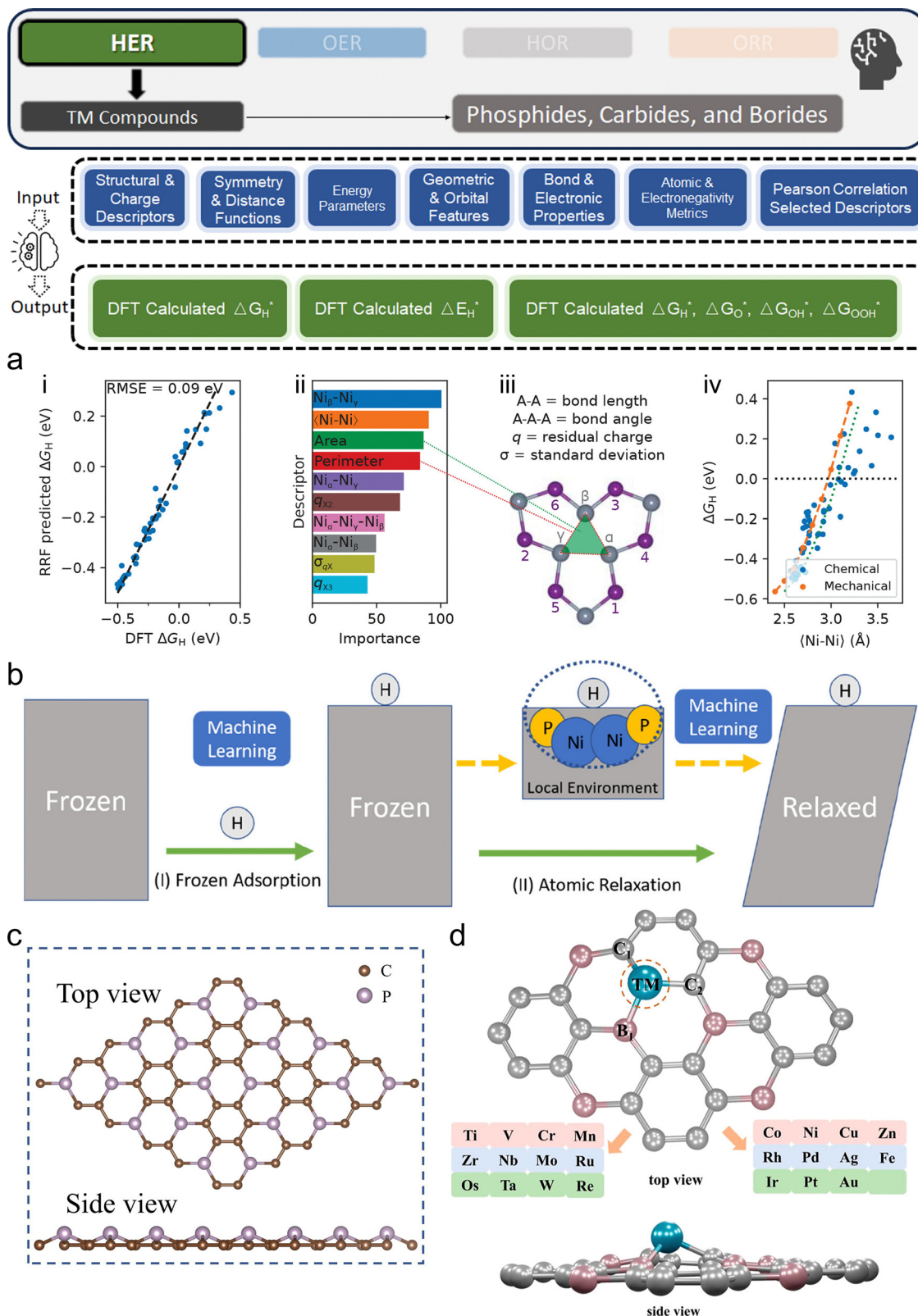
Fig. 13 (a) (i) \Delta G_{\text{H}}^* predictions by the regularized RF versus DFT: the black-dashed line indicates perfect correlation. (ii) Top 10 descriptors' relative importance from the model. (iii) Descriptor definitions: The three Ni atoms closest to the first doping site are labeled \alpha , \beta , and \gamma , based on proximity. (iv) Impact on \Delta G_{\text{H}}^* by Ni-Ni bond length: the role of chemical (via nonmetal doping) and mechanical pressure (by immobilizing surface Ni atoms), identifying the optimal Ni-Ni bond length for HER as 2.97 to 3.07 Å, with adjustments for bond contraction upon H adsorption, highlighted by a green dotted line (reproduced from ref. 179 with permission). (b) Workflow of the proposed stepwise strategy for predicting adsorption energy E_{\text{H}} on amorphous catalyst surfaces using ML: this includes two key stages – (I) calculating frozen adsorption energy, where the initial adsorption energy is estimated without considering atomic rearrangements, and (II) determining structural relaxation energy, which accounts for the energy changes resulting from structural adjustments upon adsorption (reproduced from ref. 180 with permission). (c) Schematic structure of 3 \times 3 \text{ PC}_3 monolayer (reproduced from ref. 185 with permission). (d) Top and side views of the TM/C3B monolayer structure (reproduced from ref. 186 with permission).
