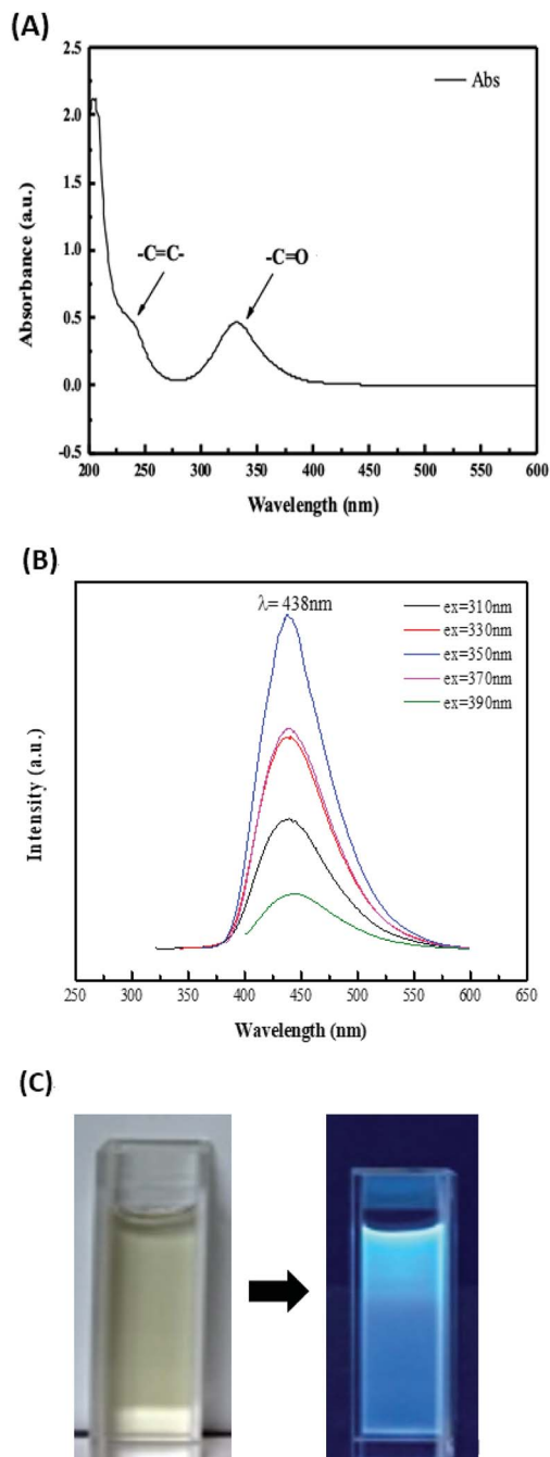
Fig. 3 (A) UV-vis absorption spectrum of CDs. (B) Fluorescence emission spectra of CDs under varied excitation wavelengths. (C) Photographs of CDs under daylight (left) and a UV lamp (365 nm, right).
