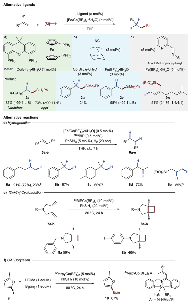
Scheme 3 Application of tetrafluoroborate activation to other ligand classes for alkene hydroxylation (top). Reaction conditions: (a) xantphos or dpfp (1 mol%), Co(BF_4)_2 \cdot 6H_2O (1 mol%), 1-octene (1 mmol), phenylsilane (1.1 mmol), THF (2 M), r.t., 4 h. (b) Adamantyl isocyanide (9 mol% [Co] or 6 mol% [Fe]), metal tetrafluoroborate (3 mol%), \alpha -methylstyrene ([Co], 1 mmol) or styrene ([Fe], 1 mmol), phenyldimethylsilane (1.3 mmol), THF (2 M), 80 °C, 3 h. (c) iPrIP (5 mol%), Fe(BF_4)_2 \cdot 6H_2O (5 mol%), myrcene (1 mmol), triethoxysilane (1.2 mmol), THF (2 M), r.t., 16 h. (d) Alkene (1 equiv.), Co(BF_4)_2 \cdot 6H_2O (0.5 mol%), Me^{es}BIP (1 mol%), PhSiH_3 (5 mol%), H_2 (20 bar), r.t., 7 h. ^{\ddagger} Alkene (1 equiv.), Fe(BF_4)_2 \cdot 6H_2O (2 mol%), Me^{es}BIP (2 mol%), PhSiH_3 (5 mol%), H_2 (20 bar), r.t., 7 h. ^{\S} Co(BF_4)_2 \cdot 6H_2O (1 mol%) and Me^{es}BIP (1 mol%). (e) 1,6-Diene (1 equiv.), EtBIPCo(BF_4)_2 \cdot 6H_2O (10 mol%), PhSiH_3 (20 mol%), 80 °C, 24 h. (f) Arene (15 equiv.), (4-NMe_2-Ph-terpy)Co(BF_4)_2 (5 mol%), PhSiH_3 (20 mol%), LiOMe (1 equiv.), B_2pin_2 (1 equiv.), 80 °C, 24 h.
