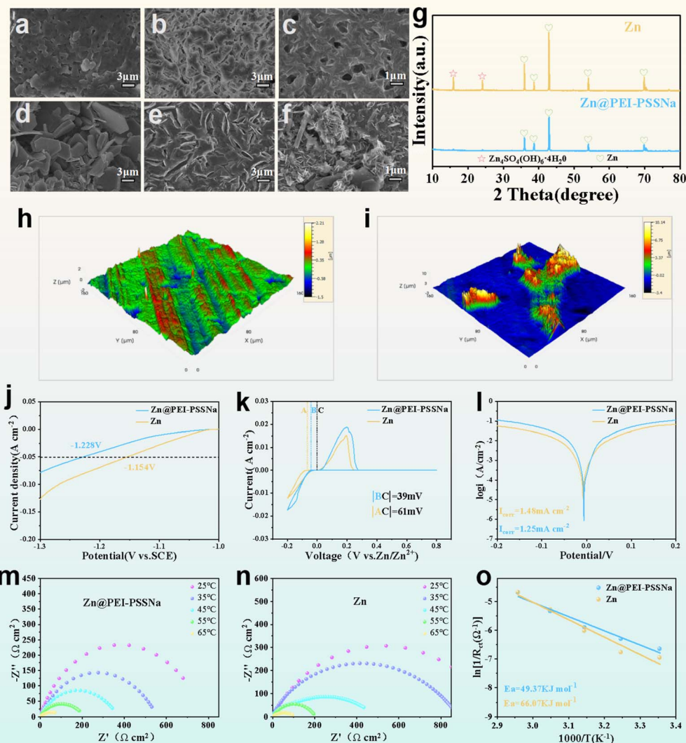
Fig. 3 SEM images of (a) Zn@PEI-PSSNa and (d) bare Zn after 50 cycles in a symmetric cell at 1\text{ mA cm}^{-2} and 1\text{ mAh cm}^{-2} . SEM images of (b) Zn@PEI-PSSNa and (e) bare Zn after 30 days of immersion in 2 M \text{ZnSO}_4 . Scanning electron microscopy images of (c) Zn@PEI-PSSNa and (f) bare Zn after 50 cycles in a Zn||Cu cell at a current density of 1\text{ mA cm}^{-2} and 1\text{ mAh cm}^{-2} . (g) Comparison of XRD images after 50 cycles at 1\text{ mA cm}^{-2} and 1\text{ mAh cm}^{-2} . HRCM images of (h) Zn@PEI-PSSNa and (i) bare Zn after 50 cycles at 1\text{ mA cm}^{-2} and 1\text{ mAh cm}^{-2} . (j) LSV testing of materials. (k) CV curve of the Zn||Cu cell. (l) Tafel curves for samples. Nyquist plots of (m) Zn@PEI-PSSNa and (n) bare Zn at different temperatures. (o) Arrhenius curve corresponding to the sample.
