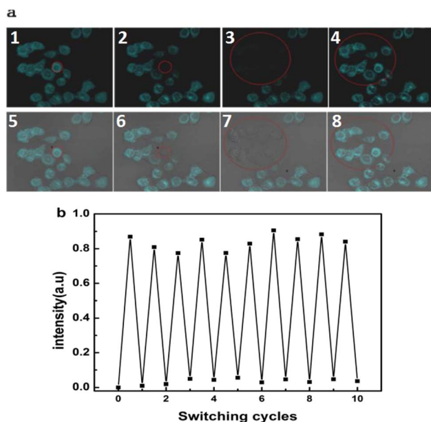
Fig. 3 (a) CLSM image (above) and the overlay image (bottom) of fixed HeLa cells incubated with 20 \mu\text{M} BMBT for 30 min at 37 ^{\circ}\text{C} (1) and (5) in original state; (2) and (6) irradiated by 488 nm light (0.5 mW) for a single cell; (3) and (7) all cells, and; (4) and (8) recovered by 405 nm light (1.25 mW). (b) Fluorescence switching of fixed HeLa cells by alternating UV (405 nm, 1.25 mW, 10 s/time) and visible (488 nm, 0.5 mW, 3 min/time) light illumination ( \lambda_{\text{ex}} = 405 \text{ nm} ).
