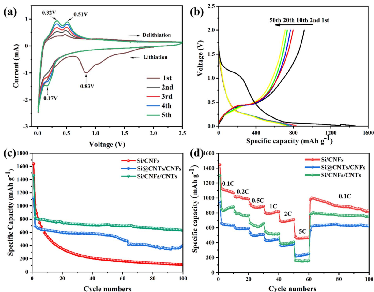
Fig. 7 (a) CV curves of Si/CNFs/CNTs at first five cycles, (b) charge–discharge curve of Si/CNFs/CNTs at different cycles, (c) cycling performance at 100 \text{mA g}^{-1} and (d) rate performance of Si/CNFs, Si@CNTs/CNFs and Si/CNFs/CNTs.
