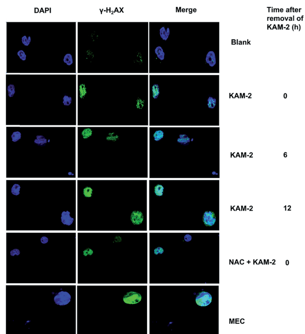
Fig. 7 Immunofluorescence of DNA cleavage protein γ-H 2 AX. HL-60 cells were treated with KAM-2 or MEC (10 μM) for 12 h, or pre-incubated with ROS scavenger NAC (20 mM) for 1 h, followed by treatment with KAM-2 for 12 h. For some groups, cells were incubated for an additional 6 or 12 h after removal of KAM-2.
