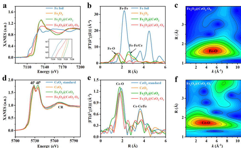
Fig. 2 XAFS characterization. (a) Fe K-edge XANES spectra and (b) Fourier-transformed k^3 -weighted EXAFS spectra of \text{Fe}_2\text{O}_3@ \text{CeO}_2\text{-O}_\text{V} , \text{Fe}_2\text{O}_3@ \text{CeO}_2 , \text{Fe}_2\text{O}_3 and Fe foil as reference. (c) WT-EXAFS contour plot of Fe K-edge signals of \text{Fe}_2\text{O}_3@ \text{CeO}_2\text{-O}_\text{V} . (d) Ce \text{L}_3 -edge XANES spectra and (e) Fourier-transformed k^2 -weighted EXAFS spectra of \text{Fe}_2\text{O}_3@ \text{CeO}_2\text{-O}_\text{V} , \text{Fe}_2\text{O}_3@ \text{CeO}_2 , \text{CeO}_2 and commercial \text{CeO}_2 as reference. (f) WT-EXAFS contour plot of Ce \text{L}_3 -edge signals of \text{Fe}_2\text{O}_3@ \text{CeO}_2\text{-O}_\text{V} .
