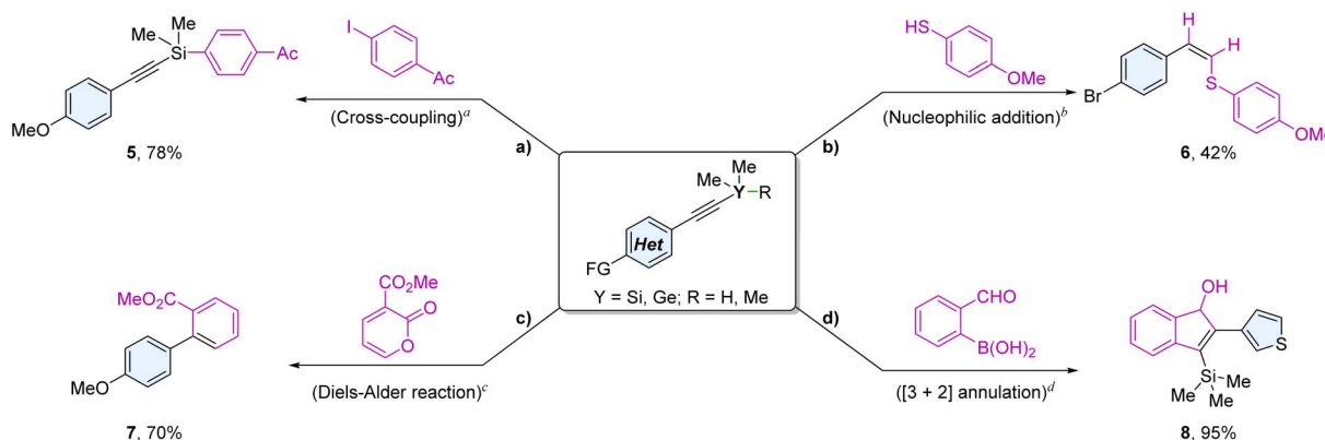
Fig. 4 Derivatization of alkynylsilanes/alkynylgermanes. Reaction conditions: a 1-(4-iodophenyl)ethan-1-one (0.15 mmol), 3a (2 equiv.), Pd(OAc) 2 (4 mol%), LiCl (4 equiv.), pyridine (2.4 equiv.), DMI, r.t. b 3p (0.15 mmol), 4-methoxybenzenethiol (1 equiv.), KOH (1 equiv.), DMSO, 120 °C. c 3ar (0.10 mmol), 2-pyrone (2 equiv.), ZnCl 2 (10 mol%), DCE, 140 °C. d 3v (0.15 mmol), ortho -formylphenylboronic acid (1.5 equiv.), Co(acac) 3 (10 mol%), DPPE (10 mol%), MeCN, 80 °C.
