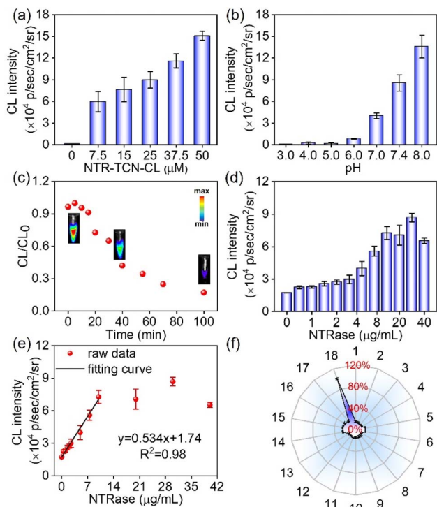
Fig. 3 (a) CL intensity of NTR-TCN-CL at varying concentrations in the presence of NTRase (10 μg mL -1 ). (b) Effect of pH on the CL intensity of NTR-TCN-CL (25 μM). (c) CL kinetics and images (inset) of NTR-TCN-CL (25 μM) following the addition of NTRase (10 μg mL -1 ). (d) CL intensity of NTR-TCN-CL upon addition of NTRase at different concentrations. (e) Linear relationship between CL intensity of NTR-TCN-CL and NTRase concentration in the range of 0–10 μg mL -1 . (f) Selectivity of NTR-TCN-CL (25 μM) toward various analytes (1: histidine, 2: lysine, 3: alanine, 4: valine, 5: serine, 6: glycine, 7: aspartic acid, 8: glutathione, 9: KCl, 10: NaHCO 3 , 11: Na 2 SO 3 , 12: FeSO 4 , 13: L-ascorbic acid, 14: NADH, 15: AzoRase, 16: HNQO1, 17: LDA, and 18: NTRase, 500 μM for 1–14; 10 μg mL -1 for 15–18). All measurements were carried out in PBS at 37 °C.
