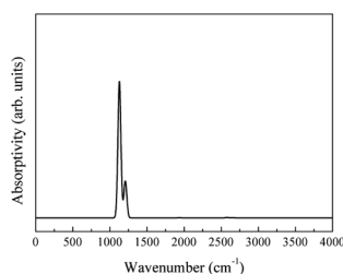
Fig. 16 Infrared spectrum of the free-carrier absorption of CeO 2 .
