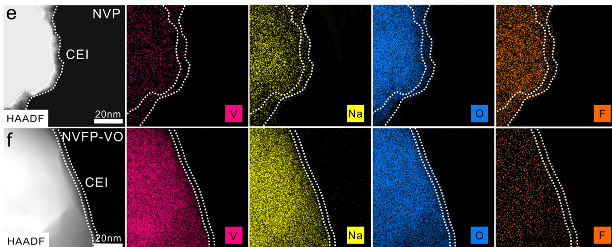
Fig. 5 Ex situ characterizations of NVP and NVFP-VO cathodes. In-depth element distributions and high-resolution XPS spectra of F 1s and C 1s. (a) and (b) NVP, and (c) and (d) NVFP-VO. HAADF-STEM and STEM-EDS mappings of (e) NVP and (f) NVFP-VO.
