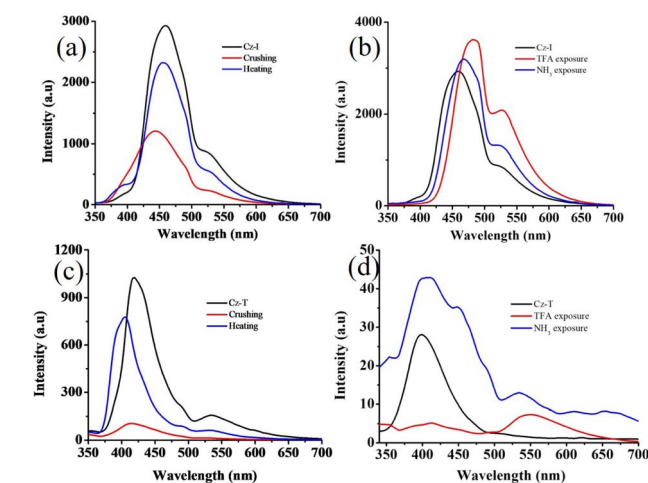
Fig. 5 (a and c) Reversible fluorescence switching of (a and b) Cz-I and (c and d) Cz-T by (a and c) crushing/heating and (b and d) TFA/ \text{NH}_3 exposure. \lambda_{\text{exc}} = 320 nm.
