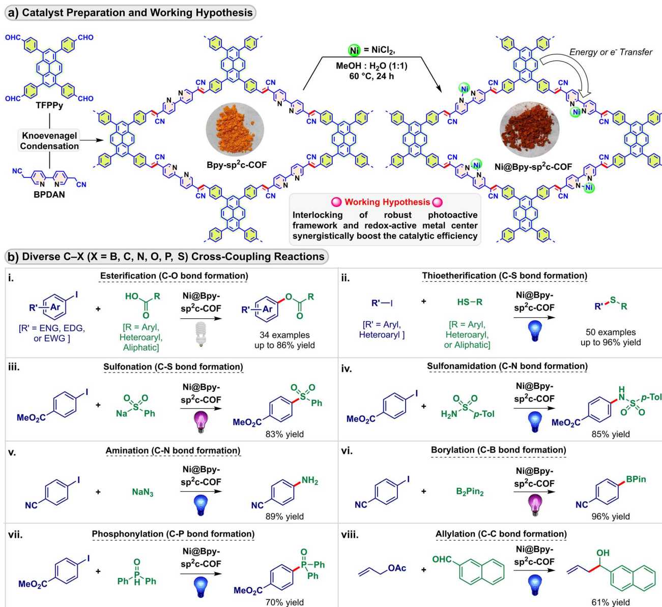
Fig. 1 (a) Catalyst preparation via \text{NiCl}_2 installation in the Bpy- \text{sp}^2\text{c-COF} and the working hypothesis; and (b) application of the Ni@Bpy- \text{sp}^2\text{c-COF} catalyst in different C–X (X = B, C, N, O, P, S) cross-coupling reactions with isolated yields of the products. ENG = electron neutral group, EDG = electron donating group, EWG = electron withdrawing group.
