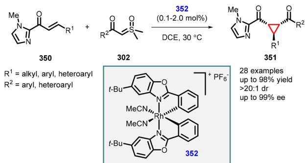
Scheme 79 Chiral Rh(III) complex-catalyzed cascade MIRC cyclopropanation of \alpha,\beta -unsaturated 2-acyl imidazoles with sulfoxonium ylides.
