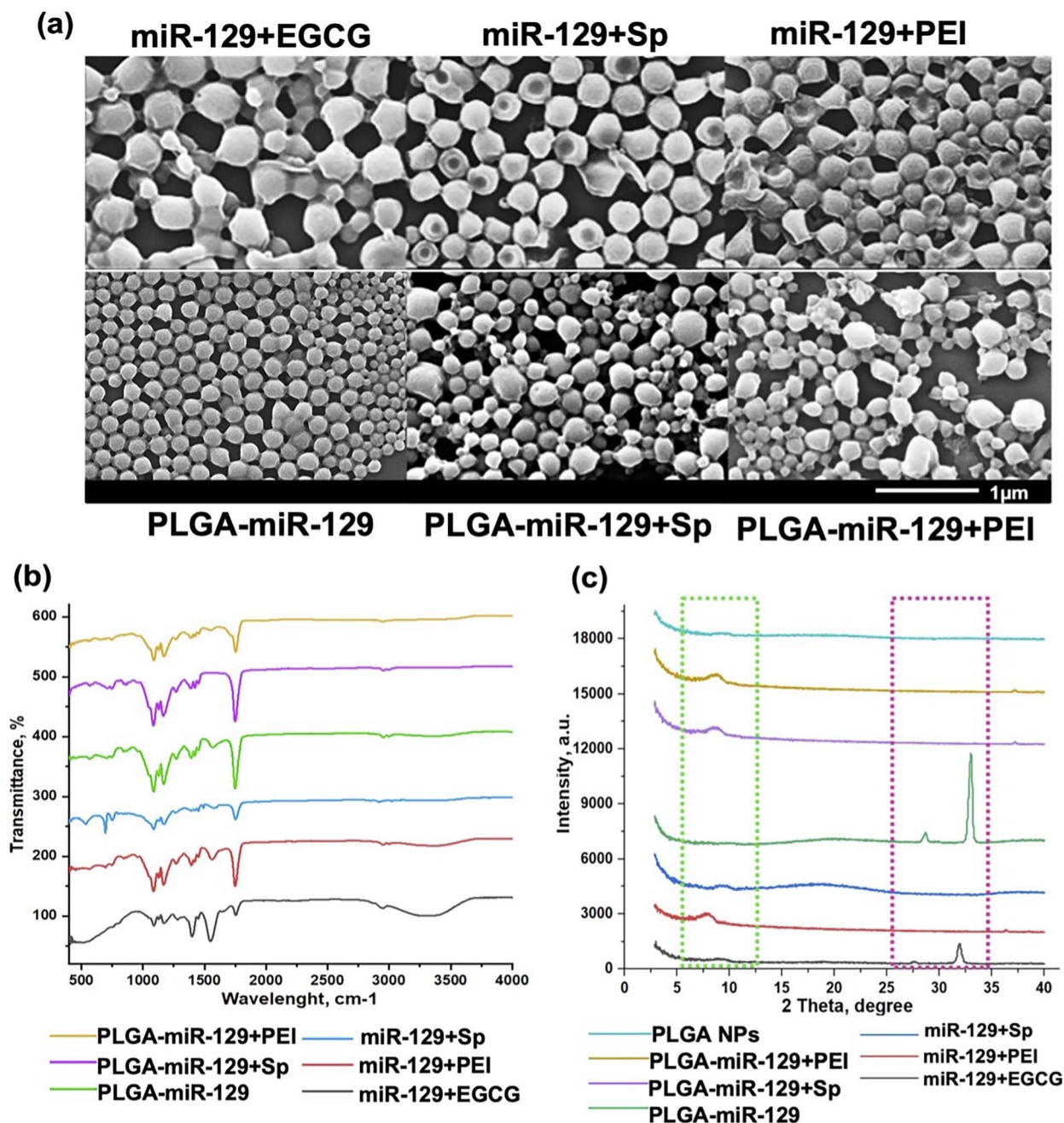
Fig. 2 NPs characterization. (a) Scanning electron microscopy (SEM) of NPs (scale bar is 1 μm, ×40k); (b) FTIR; and (c) X-ray diffraction patterns of the nanoformulations (light green dash line: PLGA and magenta dash line: miRNA). The data demonstrated PLGA-incorporated surfactant (PEMA), miR-129, and excipients. The FTIR and pXRD data for controls are presented in Fig. S1.†
