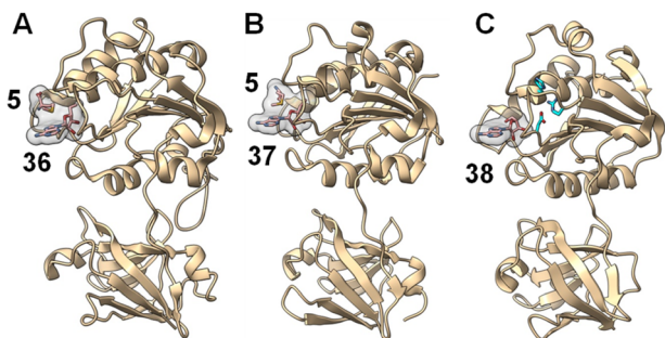
Fig. 11 A similar overall structure was observed for three adenosyl transfer enzymes. (A) The product complex between fluorinase FIA/36/5 (PDB ID: 1RQR). (B) The product complex between chlorinase SalL/37/5 (PDB ID: 2Q6I). (C) The product complex of a DUF62 protein from Pyrococcus horikoshii OT3 with 38 (PDB ID: 1WU8). SAM-derived products (i.e., 5 and 36–38) have a gray surface and the conserved His-Arg-Asp triad in DUF62 proteins is colored cyan.
