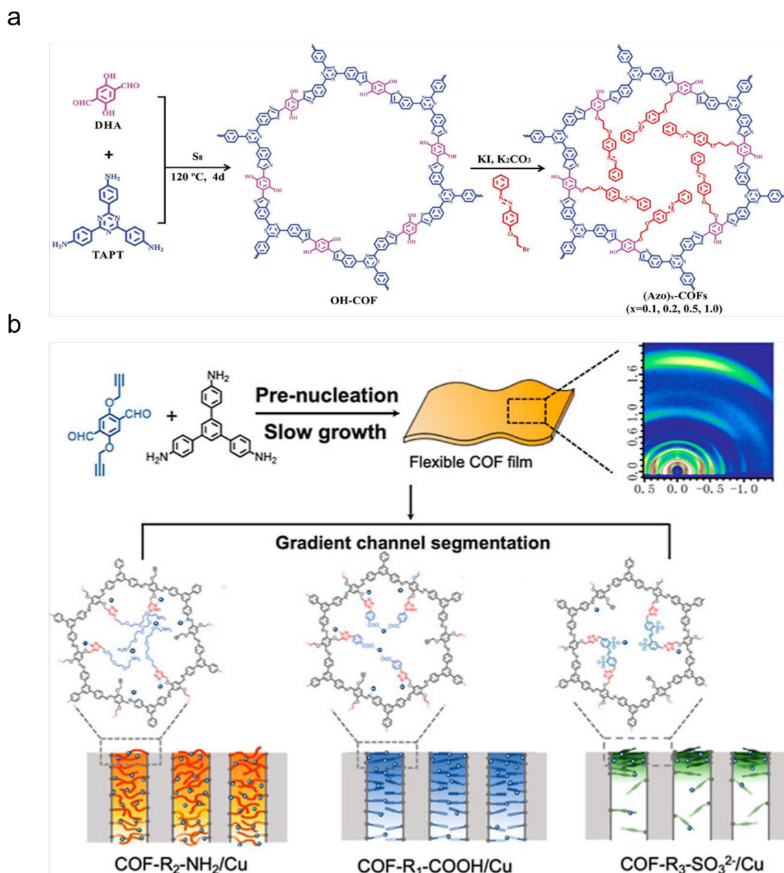
Fig. 12 a) Incorporating stimuli-responsive units through post-synthetic modification. 126 Copyright 2024, Wiley-VCH. b) Gradient channel segmentation via click reaction. 136 Copyright 2023, American Chemical Society.
