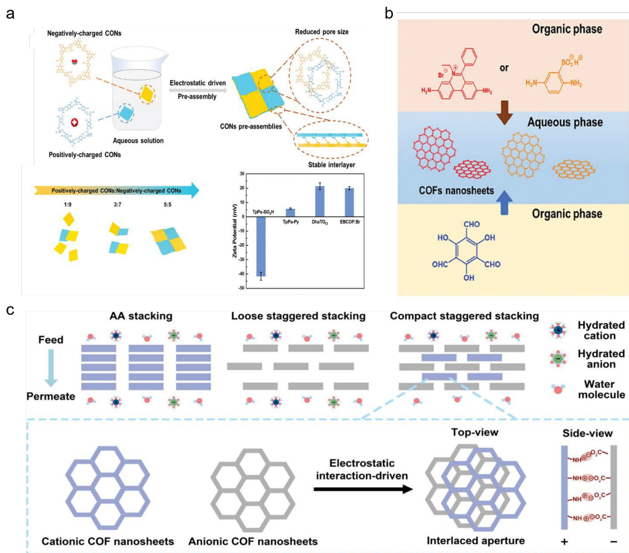
Fig. 15 a) Interlocked CONs via electrostatic interaction. 174 Copyright 2024, Wiley-VCH. b) Engineering membrane architecture with pore size mismatch and heterogeneous charges. 175 Copyright 2024, Wiley-VCH. c) Electrostatic-mediated stacking configurations of CONs. 176 Copyright 2024, American Chemical Society.
