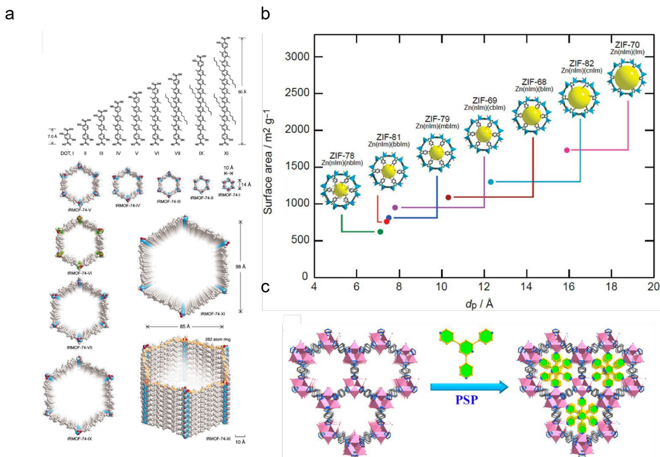
Fig. 13 a) Engineering MOF architecture via design of organic ligand. 140 Copyright 2012, The American Association for the Advancement of Science. b) Engineering MOF architecture via side chain. 141 Copyright 2009, American Chemical Society. c) Pore space partitioning through axially coordinated organic units. 144 Copyright 2019, American Chemical Society.
