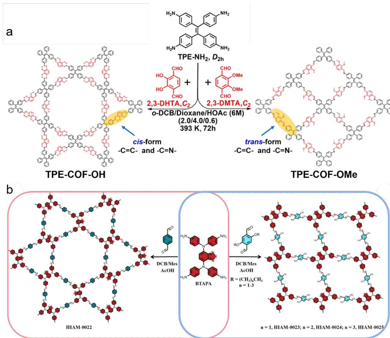
Fig. 11 a) Topological structure modulation by side-chain chemistry. 106 Copyright 2020, American Chemical Society. b) Conformational rearrangement through side-chain extension. 109 Copyright 2025, Royal Society of Chemistry.
