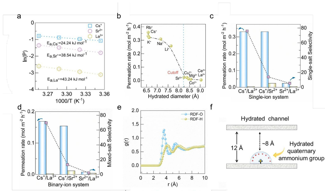
Fig. 4 Hydration layer impact on architecture and separation performance. a) Ionic conductivity experiments. b) Ion permeation rates. Rare earth element ion selectivity in c) single-salt and d) mixed-salt. e) RDF of water molecules surrounding the quaternary ammonium units. f) Schematic of effective pore size. 73 Copyright 2024, Springer.
