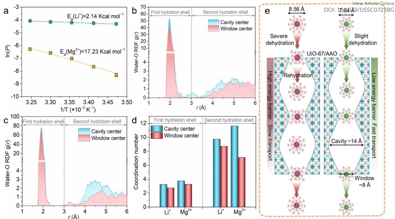
Fig. 3 Mechanistic insights into \text{Li}^+/\text{Mg}^{2+} separation. a) Ionic conductivity experiments. RDFs for: b) \text{Li}^+ and c) \text{Mg}^{2+} positioned at both cavity and window centers of UiO-67. d) First and second hydration shell of \text{Li}^+ and \text{Mg}^{2+} at diverse channel positions. e) Proposed mechanism for \text{Li}^+ and \text{Mg}^{2+} transport. 71 Copyright 2021, Wiley-VCH.
