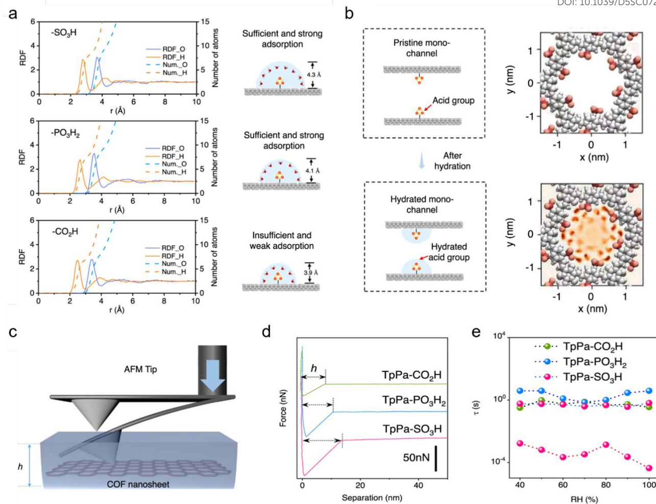
Fig. 5 Functionality impact on hydration layer thickness. a) RDF of water molecules surrounding acidic groups. b) Schematic of hydration layer impact on the structure of COF channels. c) Schematic of contact AFM measurement and its corresponding "jump-to-contact" region. d) Force-distance curve. e) Dielectric loss spectra. 74 Copyright 2022, Springer.
