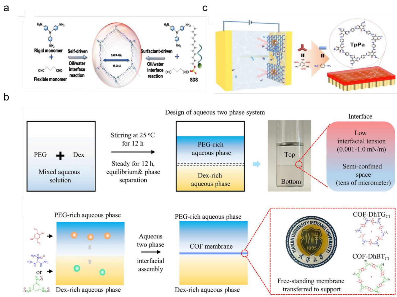
Fig. 16 a) Surfactant-assisted interface polymerization. 184 Copyright 2023, Wiley-VCH. b) Schematic of aqueous two-phase interface polymerization. 187 Copyright 2023, Wiley-VCH. c) Electrochemical interface polymerization for ultrathin COF membrane fabrication. 188
