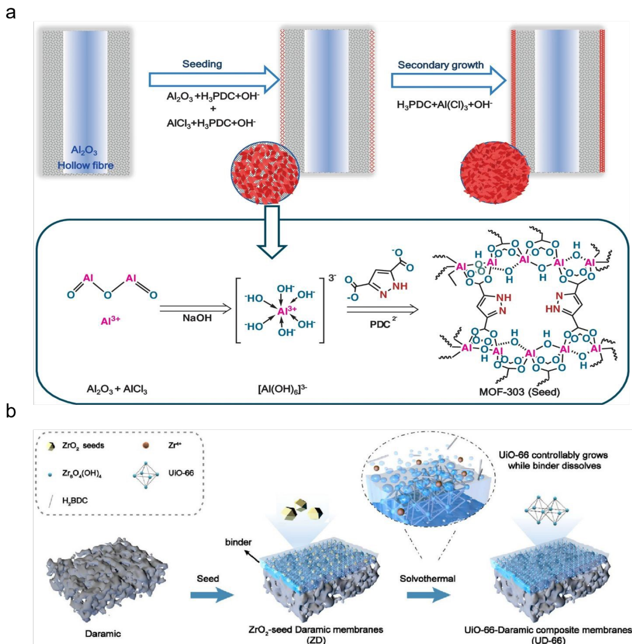
Fig. 17 a) Bimetallic-source secondary growth strategy for MOF membrane fabrication. 198 Copyright 2024, Springer. b) Seed-polymer blended to fabricate substrate for MOF membrane synthesis. 201 Copyright 2021, Elsevier.
