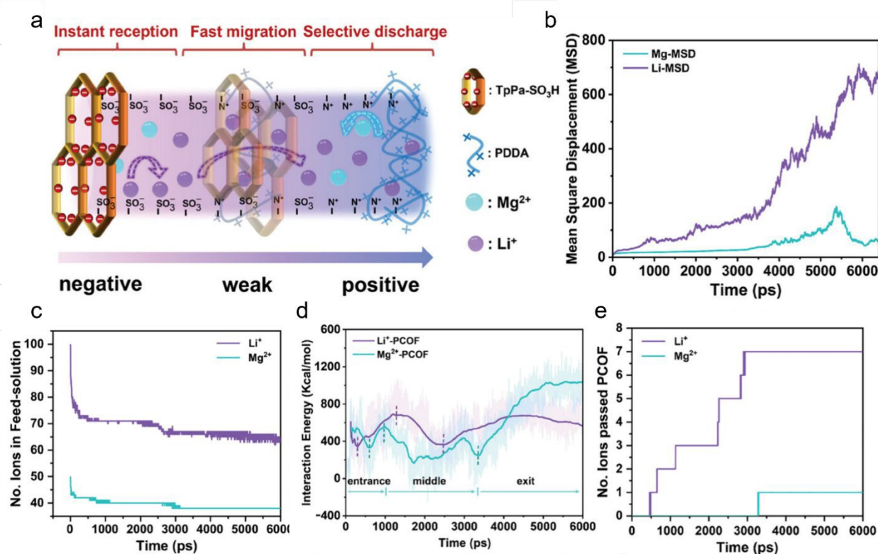
Fig. 7 Lithium-magnesium separation in heterocharged COF membranes. a) Schematic of heterocharged nanochannels. b) MSD of Mg 2+ /Li + . c) Quantity of Li + and Mg 2+ in feed-solution. d) Binding energy between ion and COF. e) Ion transport numbers across COF frameworks. 70 Copyright 2024, Wiley-VCH.
