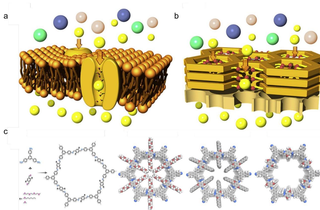
Fig. 8 Biomimetic architecture design of COF membranes. a) Schematic representation of biological ion channels. b) Schematic representation of bioinspired artificial ion channels. c) Schematic illustrations of COF structures derived from TAB reactions with various aldehyde monomers. 88 Copyright 2021, Elsevier.
