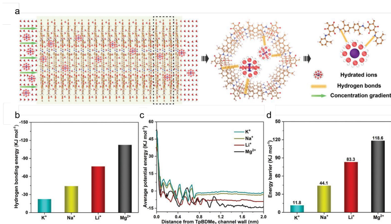
Fig. 10 Hydrogen-bonding-inspired design of COF membrane. a) Hydrogen-bond-mediated diffusion behaviour. b) Hydrogen bond energies between ions and COF. c) Average potential energy of ions. d) Energy barriers for ion transport. 92 Copyright 2021, Wiley-VCH
