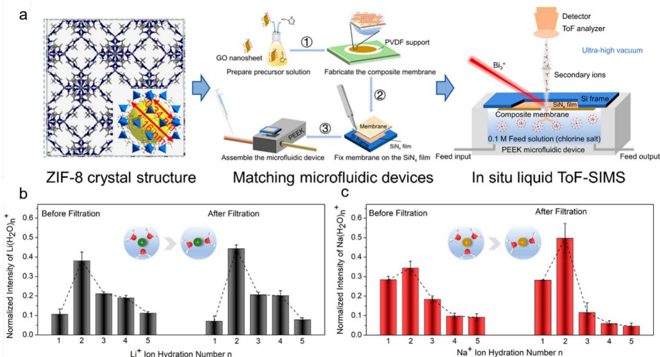
Fig. 2 Hydration structure characterization. a) Schematic of ZIF-8 structure and microfluidic technology coupled with in situ liquid ToF-SIMS analysis. The hydration structure of b) \text{Li}^+ and c) \text{Na}^+ before and after filtration. 55 Copyright 2023, American Chemical Society.
