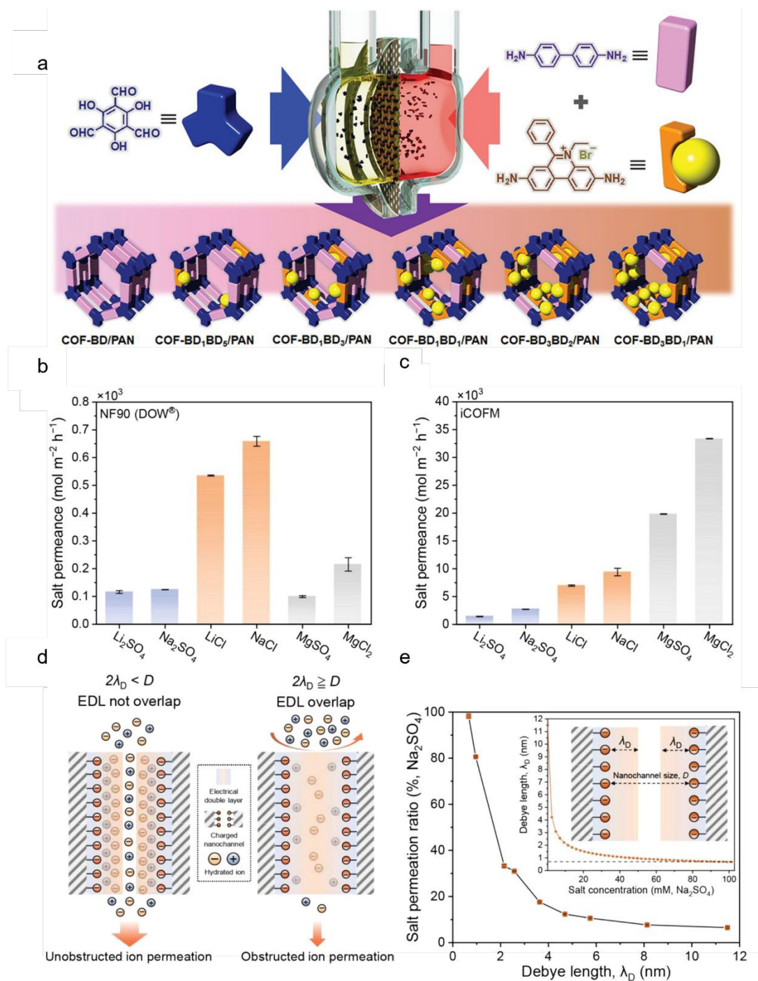
Fig. 6 a) Schematic of charge density modulation through precise monomer ratio control. 57 Copyright 2021, Wiley-VCH. Ion transport behavior governed by the electric double-layer. Salt permeation rates of b) commercial nanofiltration membranes versus c) ionic COF membranes. d) Electric double layer-governed ion diffusion behavior. e) Salt permeability under varying Debye lengths. Insets: Illustration of
