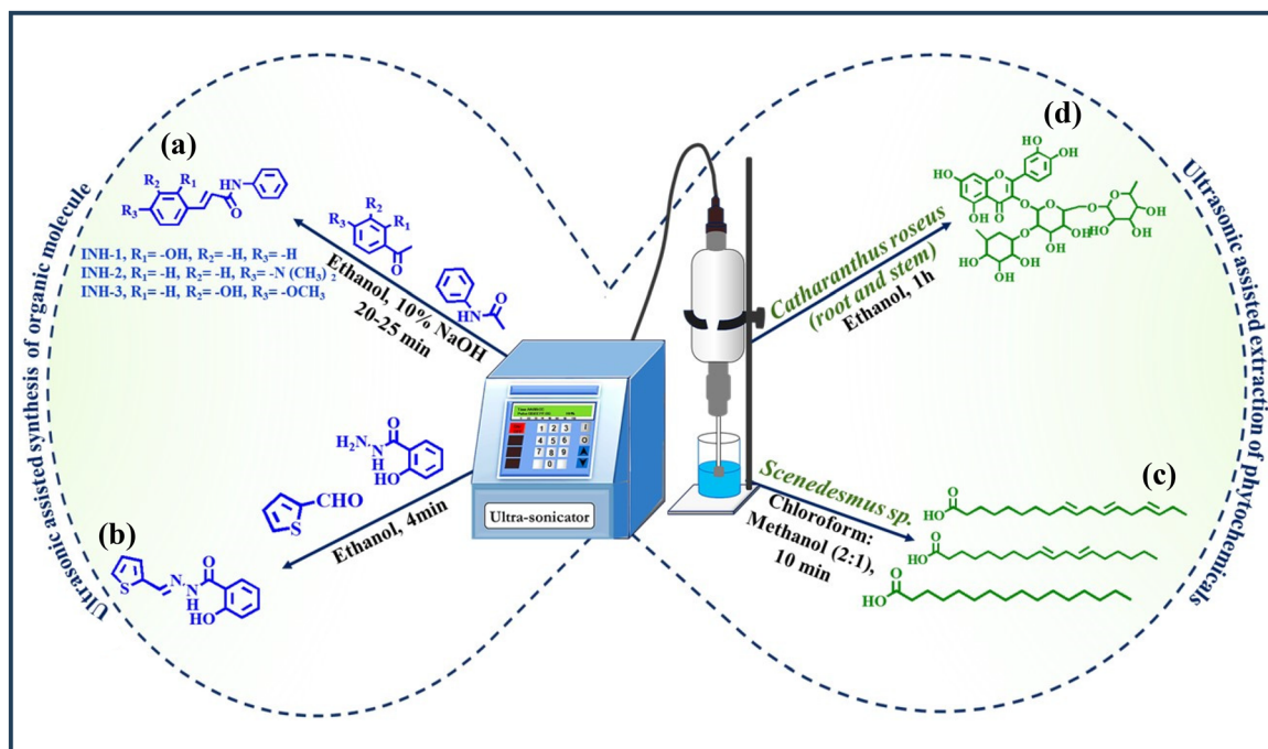
Fig. 13 Schematic presentation of the green synthetic pathways for corrosion inhibitors via the ultrasound-assisted protocol for (a) INH-1, INH-2, and INH-3 315 [reproduced from ref. 315 with permission; Copyright, Elsevier, 2014]; (b) HTMBH 316 [reproduced from ref. 316 with permission; Copyright, ACS, 2018]; (c) Scenedesmus sp. extract 317 [reproduced from ref. 317 with permission; Copyright, ACS, 2018]; and (d) Catharanthus roseus extract 318 [reproduced from ref. 318 with permission; Copyright, RSC, 2020].
