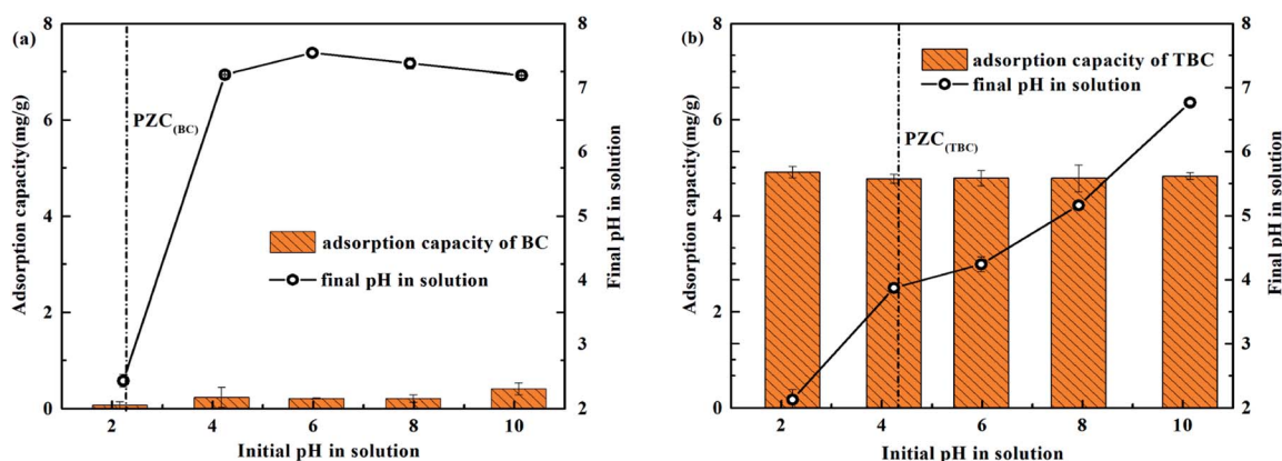
Fig. 6 Effect of initial solution pH on the adsorption capacity for As(III) removal by BC (a) or TBC (b) at As(III) initial concentration of 10 \text{ mg L}^{-1} .
