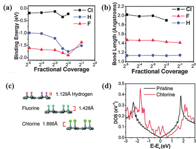
Fig. 14 (a) Binding energies and (b) bond lengths of the C–X bond ( X = \text{Cl}, \text{H}, \text{F} ) as functions of coverage, based on ab initio simulations. (c) Atomistic structures and bond lengths of C–X. (d) Calculated DOS of graphene with a 1/30 coverage of Cl atoms in comparison with that of pristine graphene as a function of energy E - E_F , where E_F is the Fermi energy. Adapted with permission from ref. 111. Copyright (2011) American Chemical Society.
