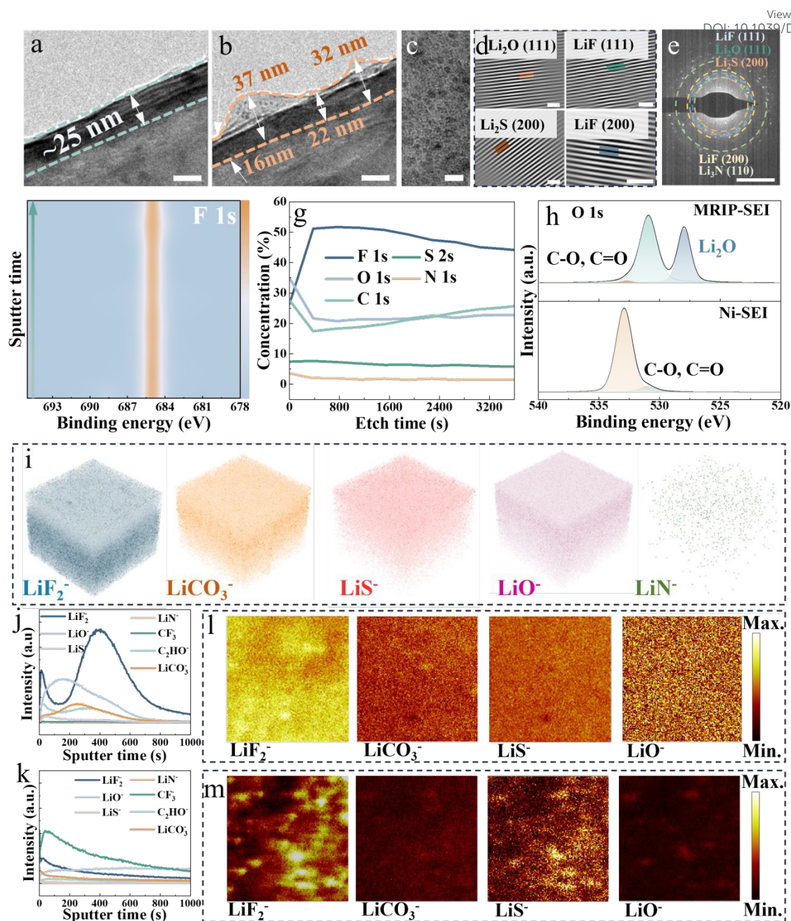
Fig. 3 Composition distribution of MRIP-SEI layer induced by HCMAS. Cryo-TEM images of (a) MRIP-SEI (M-Ni) and (b) Ni-SEI morphologies (Scale bar: 20 nm). (c) High-resolution Cryo-TEM images of the MRIP-SEI (Scale bar: 5 nm). (d) Inverse FFT images of MRIP-SEI (Scale bar: 1 nm). (e) SAED pattern of the regions at the surface of growth lithium (Scale bar: 5 1/nm). (f) High-resolution XPS spectra depth-profiles of the formed MRIP-SEI (M-Ni) of F 1s. (g) The atomic composition ratios of MRIP-SEI varying with sputter time. (h) XPS spectra of O 1s of MRIP-SEI and Ni-SEI. (i) TOF-SIMS 3D distribution of MRIP-SEI (M-Ni). Depth profiles of (j) MRIP-SEI and (k) Ni-SEI. Single-color gradient maps of \text{LiF}_2^- , \text{LiCO}_3^- , \text{LiS}^- , and \text{LiO}^- in (l) MRIP-SEI and (m) Ni-SEI.
