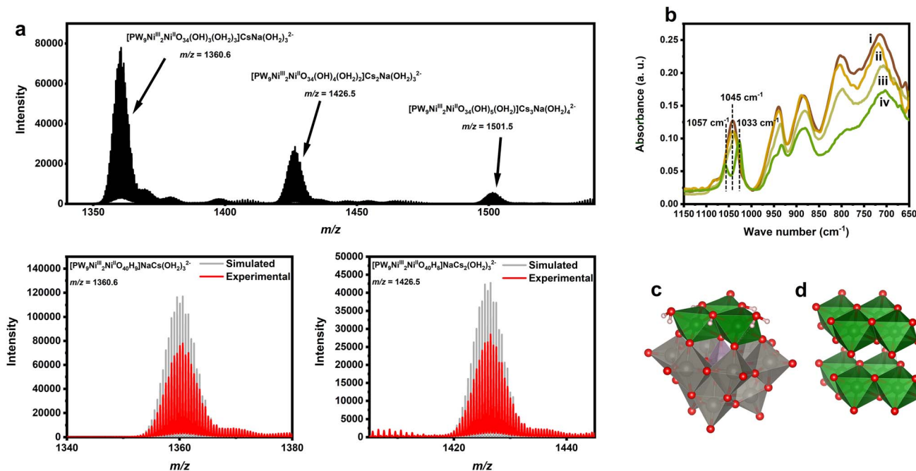
Fig. 1 (a) ESI mass spectrum of aqueous solution of Cs 4 K-1. Simulation for peaks at m/z = 1360.6 and 1426.5 is shown for comparison. (b) IR spectrum of the freshly prepared (i) and partially reduced (ii and iii) Cs 4 K-1 sample and reduced Cs 4 KH-2 sample (iv). (c) Polyhedral structural representation of the computed most stable isomer B-α-1. (d) The crystal structure of Ni(OH) 2 . 50
