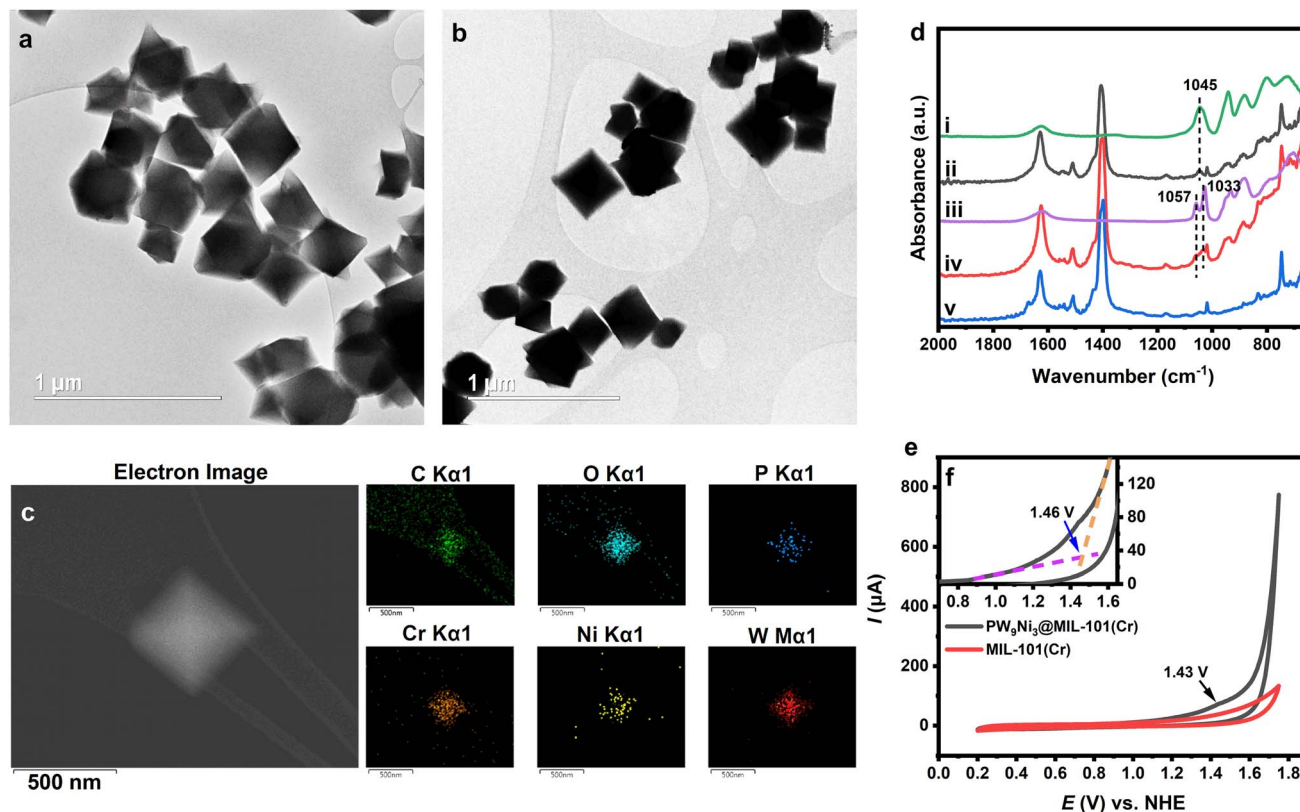
Fig. 4 (a) Bright-field-conventional transmission electron microscopy (BF-CTEM) images of the \text{PW}_9\text{Ni}_3/\text{MIL-101(Cr)} composite. (b) (BF-CTEM) images of MIL-101(Cr) particles. (c) Dark-field-scanning transmission electron microscopy (DF-STEM) image of a \text{PW}_9\text{Ni}_3/\text{MIL-101(Cr)} crystallite with the corresponding energy-dispersive X-ray spectroscopy (EDS) mapping result of the composite carbon (C), oxygen (O), phosphorus (P), chromium (Cr), nickel (Ni) and tungsten (W). (d) Comparison of IR spectra of \text{Cs}_4\text{K-1} (i), the \text{PW}_9\text{Ni}_3/\text{MIL-101(Cr)} composite after 20 min of sonication (ii), \text{Cs}_4\text{KH-2} (iii), the composite after 24 hours of stirring (iv) and MIL-101(Cr) (v). (e) Cyclic voltammogram (CV) of the \text{PW}_9\text{Ni}_3/\text{MIL-101(Cr)} composite and MIL-101(Cr) in 0.5 M \text{Na}_2\text{SO}_4 solution. (f) Illustration of the calculation of the onset potential of the \text{PW}_9\text{Ni}_3/\text{MIL-101(Cr)} composite.
