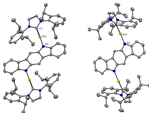
Fig. 1 Crystal structure of PhotAu3 , containing two different conformations of the PhotAu3 molecule. Thermal displacement ellipsoids are shown at the 50% probability level. Selected bond distances (Å): Au1–N1 = 1.978(4), Au1–C1 = 2.003(4), Au2–N2 = 1.976(4), Au2–C2 = 2.005(3). CCDC number: 2465569.
