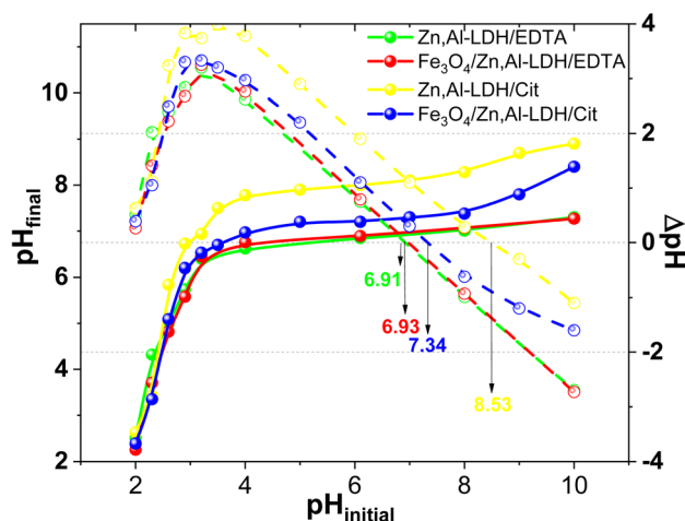
Fig. 9 The determination of pH_{pzc} of obtained adsorbents (conditions: m = 0.025 \text{ g} , V = 50 \text{ mL} , time 24 h, C(\text{NaClO}_4) = 0.1 \text{ M} ).
