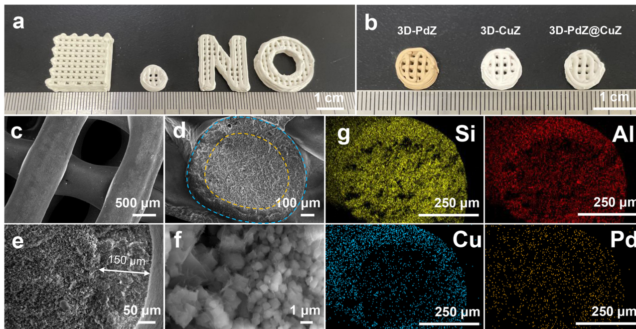
Fig. 2 (a) Digital photographs of 3D-PdZ@CuZ monoliths with different structures. (b) Digital photographs of 3D-PdZ, 3D-CuZ, and 3D-PdZ@CuZ catalysts. SEM images of 3D-PdZ@CuZ from top view (c) and cross-sectional view (d–f) at different magnifications. (g) Scanning electron microscopy energy dispersive X-ray spectroscopy (SEM-EDS) elemental mapping images of a representative cross-sectional 3D-PdZ@CuZ monolith (yellow: Si, red: Al, blue: Cu, and orange: Pd).
