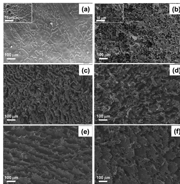
Fig. 1 TFSEM images of the PAAc hydrogel (a) and the cryogels of PAAc (b), PAAc-PANI (c), PAAc-PPy (d), PAAc-GO (e), and PAAc-rGO (f).
