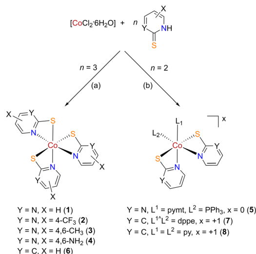
Scheme 2 Synthetic schemes and structures of complexes [\text{Co}(\text{L}^{\text{NS}})_3] and [\text{Co}(\text{L}^{\text{NS}})_2\text{L}^1\text{L}^2]^x+ (1–8): (a) (\text{CH}_3\text{CH}_2)_2\text{NH} , 50–70 °C for 3 h under atmospheric conditions, and (b) KOH or (\text{CH}_3\text{CH}_2)_2\text{NH} or \text{CH}_3\text{ONa} , 50–70 °C for 2 h under atmospheric conditions.
