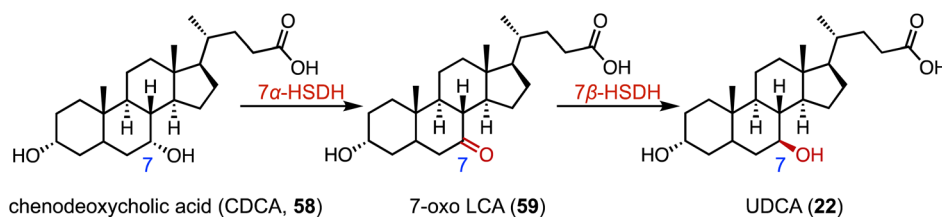
Fig. 10 The synthesis of UDCA (22) through C-7 hydroxylation mediated by 7 \alpha -HSDH and 7 \beta -HSDH.
