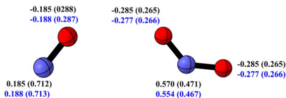
Fig. 3 Natural charge and spin population (in parantheses) of NO • (left) and NOO • (right) radical in water (black) and pentyl ethanoate (blue) at the M06-2X/6-311++G(d,p) level of theory.
