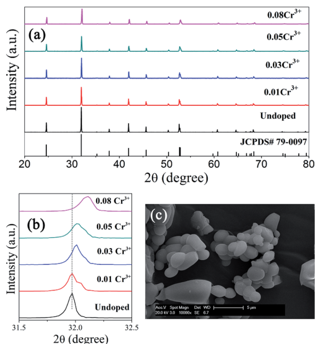
Fig. 3 (a) XRD patterns of \text{ScBO}_3:\text{Cr}^{3+} phosphors with various x values, together with the standard pattern of a rhombohedral \text{ScBO}_3 structure (JCPDS Card no. 79-0097) for comparison; (b) magnified XRD peak at \sim 32^\circ ; (c) SEM image of \text{ScBO}_3:0.02\text{Cr}^{3+} (scale bar: 5 \mu\text{m} ).
