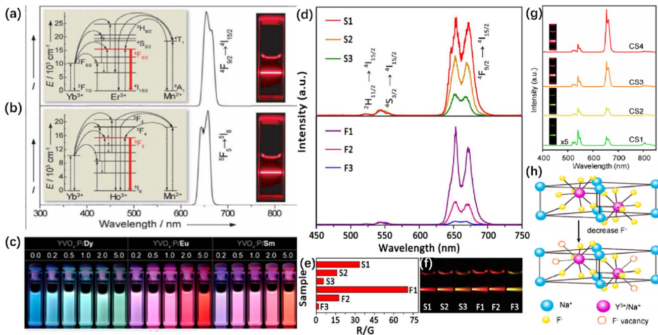
Fig. 7 Host-assisted multicolor tuning in Ln UCNCs. Room temperature UC emission spectra of (a) \text{KMnF}_3 :Yb/Er (18 : 2 mol%) and (b) \text{KMnF}_3 :Yb/Ho (18 : 2 mol%) solution. Insets are the mechanisms responsible for the single-band red emission as well as the corresponding luminescent images, recorded under excitation from a 980 nm CW diode laser with a power density of 10 \text{ W cm}^{-2} . 102 Copyright 2011, Wiley-VCH. (c) Luminescent images of \text{YVO}_4 NCs doped with phosphorus ions and different concentrations of \text{Dy}^{3+} , \text{Eu}^{3+} , and \text{Sm}^{3+} . Reproduced with permission. 7 Copyright 2014, American Chemical Society. (d) UC emission spectra of NCs upon 980 nm excitation with a power density of 10 \text{ W cm}^{-2} . (e) R/G ratios and (f) digital photographs of samples. 80 Copyright 2015, American Chemical Society. (g) UC emission spectra and corresponding luminescent photographs (insets) of the core-shell nanoparticles under 1540 nm laser excitation. (h) Schematic presentation of \text{NaErF}_4 @ \text{NaYF}_4 nanoparticles with decreasing \text{F}^- and inducing the atomic vacancies. 103 Copyright 2020, American Chemical Society.
