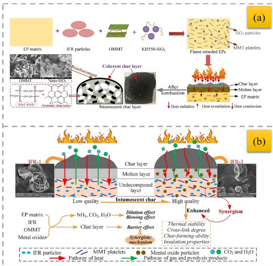
Fig. 9 Possible synergistic flame-retardant mechanism of OMMT/nano-SiO 2 for the intumescent flame-retarding EPs (a), 110 reproduced from ref. 110 with permission from John Wiley and Sons, Copyright 2020. Synergistic mechanism of IFR-OMMT-metal oxide ternary system in EPs (b), 111 reproduced from ref. 111 with permission from John Wiley and Sons, Copyright 2021.
