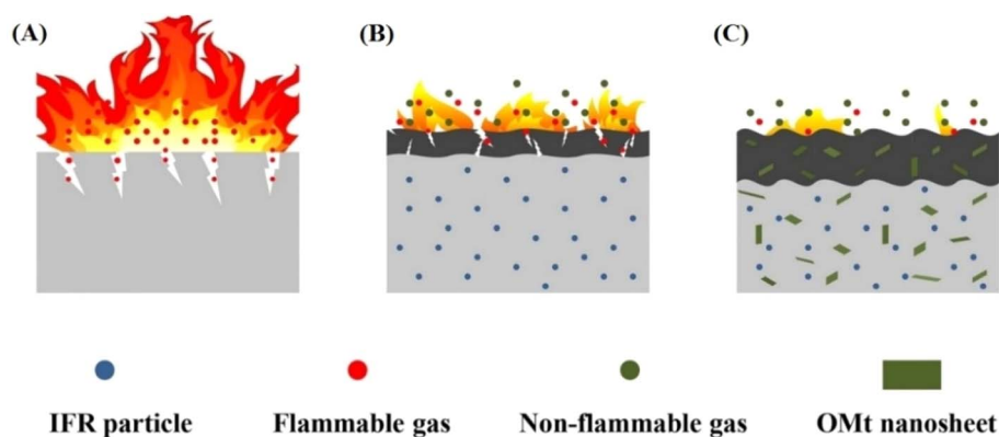
Fig. 8 Schematic of flame-retardant mechanism of (A) pure PP, (B) PP/IFR APP and (C) PP/IFR APP/OMt 100 reproduced from ref. 100 with permission from John Wiley and Sons, Copyright 2022.
